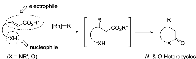
Scheme 1. Domino Conjugate Addition–Cyclization Reaction for the Synthesis of Heterocyclic Skeletons
