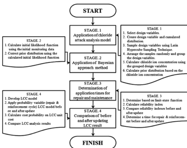
Fig. 4 Analysis procedure of durability against chloride attack and life-cycle cost
